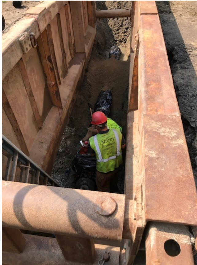
Gate Valve Installation STA 49+25.
